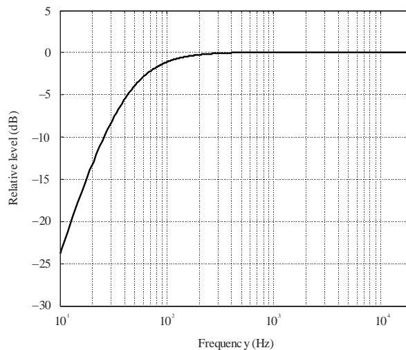
FIGURE 4 Second stage weighting curve
