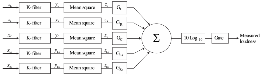
FIGURE 1 Simplified block diagram of multichannel loudness algorithm
